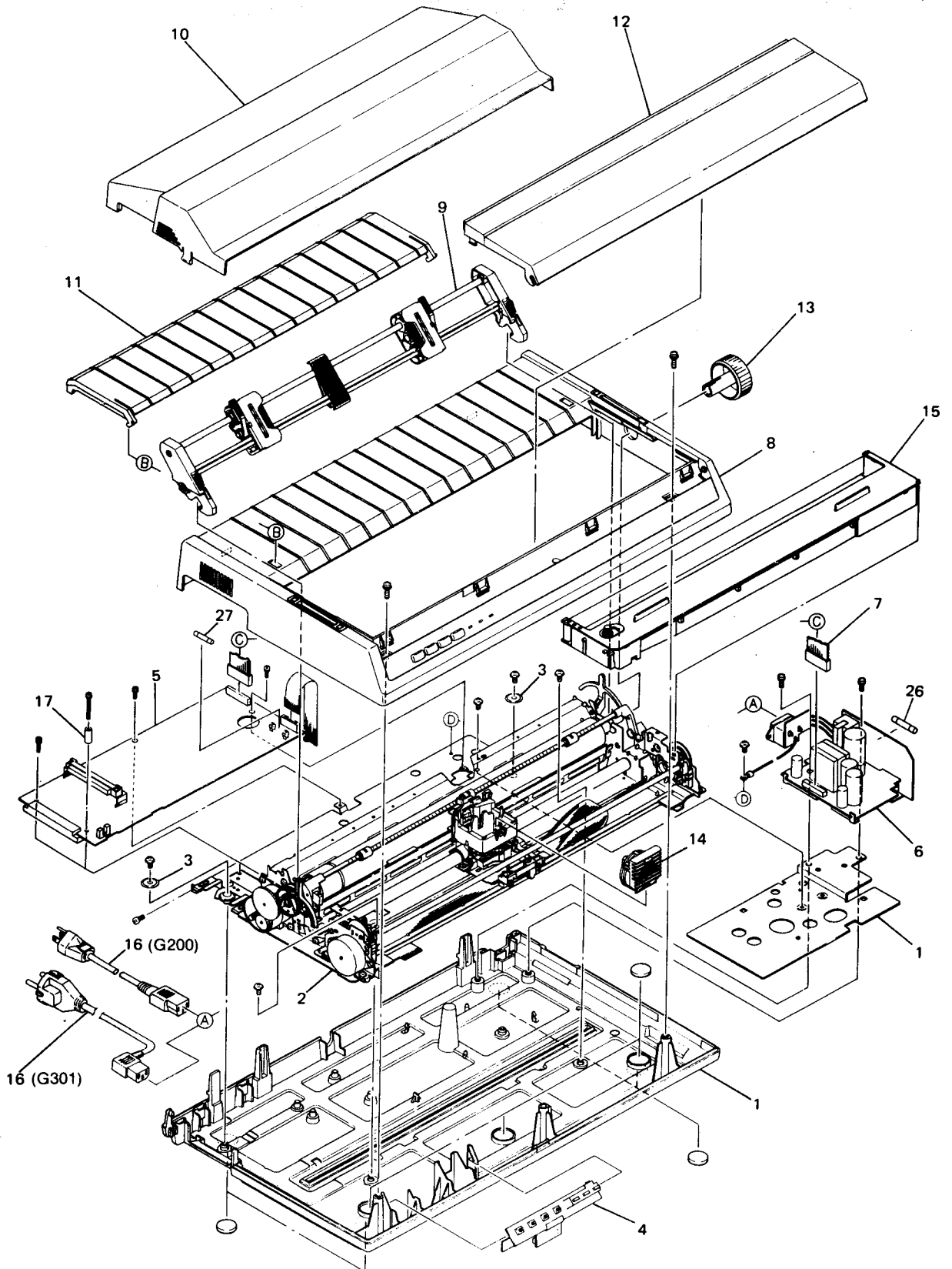
Figure 9-1 Printer unit
