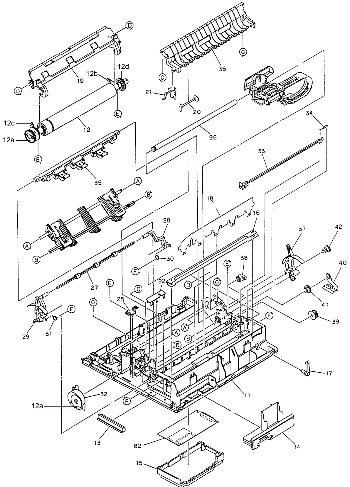
Printer unit (3/5)
