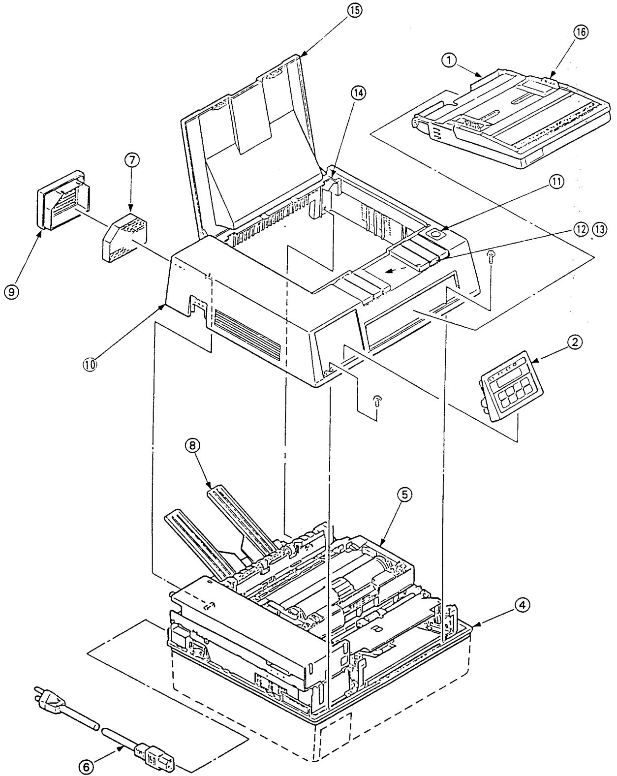
Figure 9-1 Printer unit
