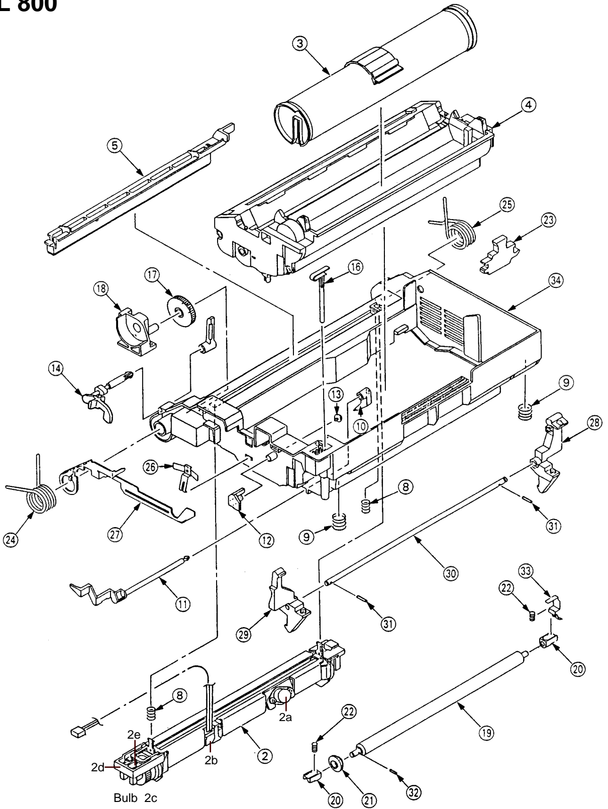
Figure 9-2 Upper unit (1/2)
