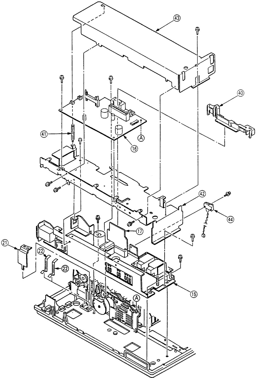
Figure 9-3 Lower unit (2/2)
