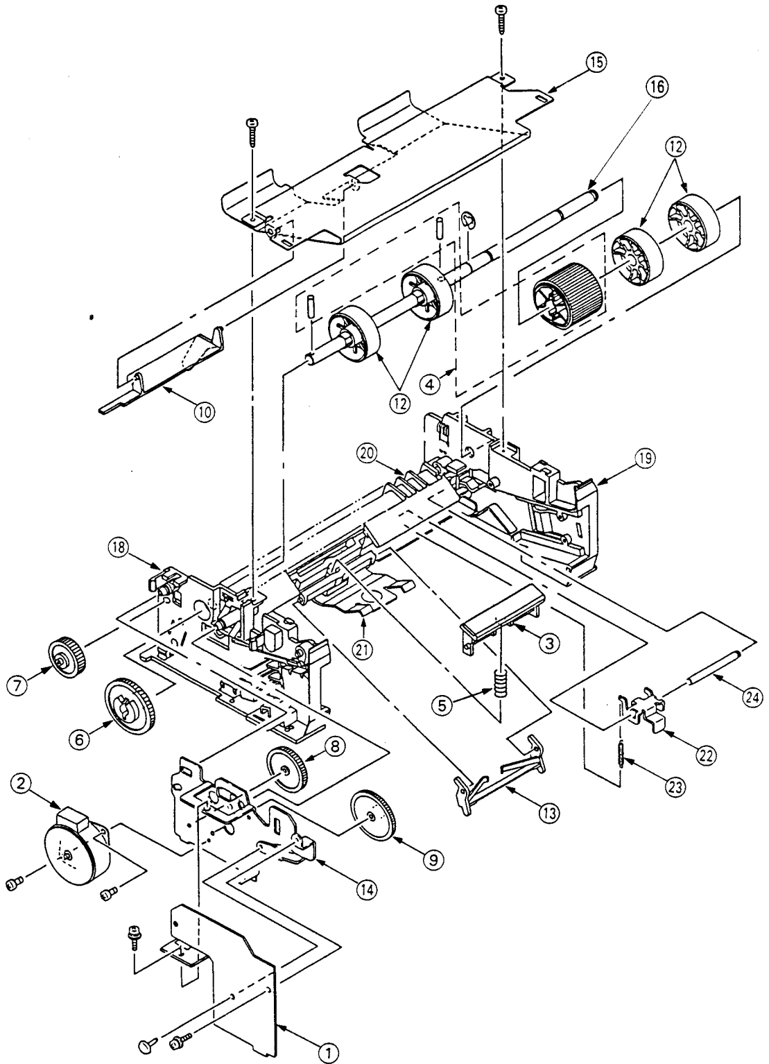
Figure 9-5 Paper supply unit
