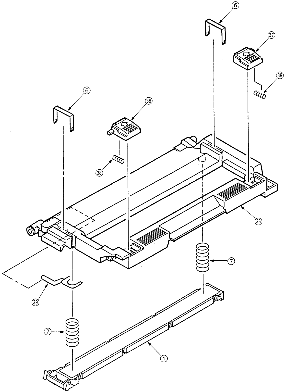
Figure 9-2 Upper unit (2/2)
