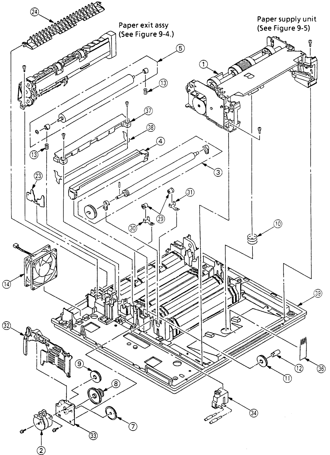
Figure 9-3 Lower unit (1/2)
